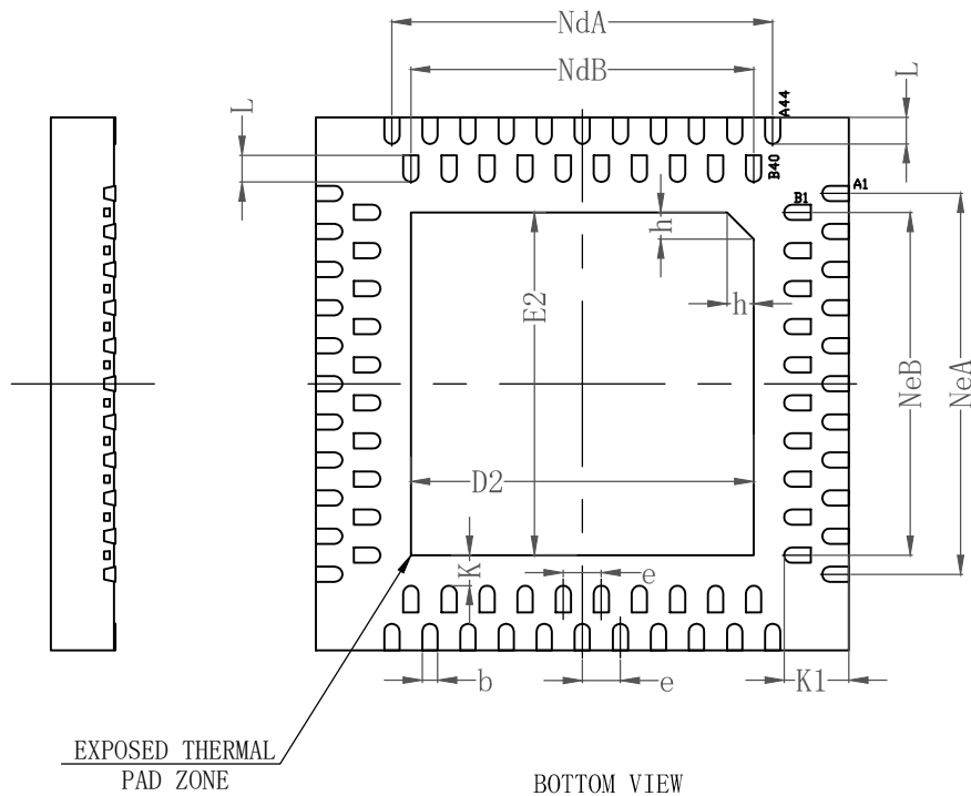
BOTTOM VIEW
